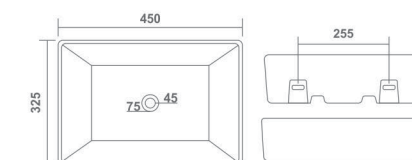
FAST L 450 W 325 H 125 mm 18" x 13"
