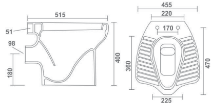
ANGLO INDIAN L 515 W 455 H 400 mm 'P' Trap
