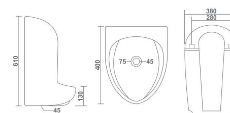
LARGE L 380 W 400 H 610 mm
