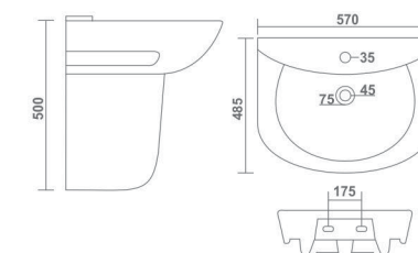
STUDIO L 570 W 485 H 500 mm 23" x 19"
