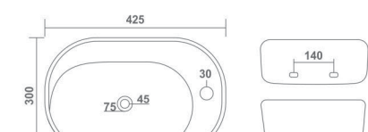
LOGAN L 425 W 300 H 145 mm 17" x 12"
