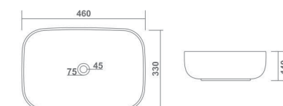
ARMIS L 460 W 330 H 140 mm 18" x 13"
