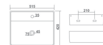
VASCA L 515 W 420 H 120 mm 21" x 17"
