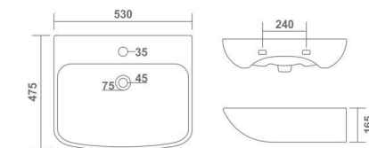
FLORIDA L 530 W 475 H 165 mm 21" x 19"
