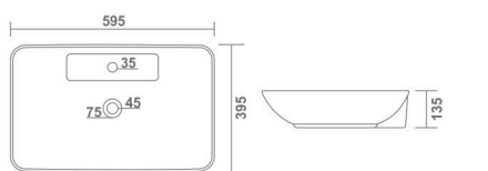
VIOLET L 595 W 395 H 135 mm 24" x 16"
