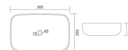
OLIVER L 365 W 255 H 105 mm 15" x 10"
