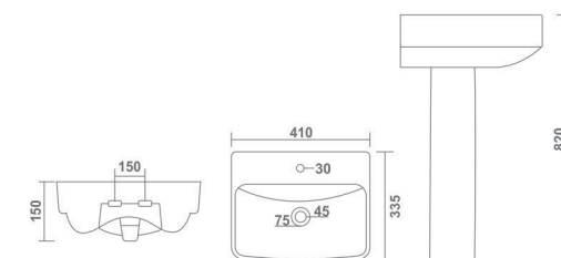
JOLLY L 410 W 335 H 820 mm 16" x 13"
