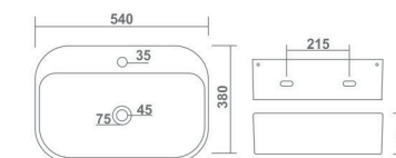
GALA L 540 W 380 H 110 mm 22" x 15"
