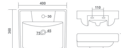
CALVIN L 400 W 360 H 160 mm 16" x 14"
