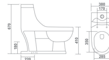
CAMRY L 700 W 380 H 670 mm 'S' Trap : 220mm (9") 'P' Trap
