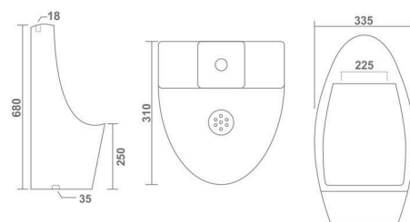
BUZZ L 335 W 310 H 680 mm
