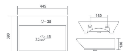
LUMINA L 445 W 390 H 130 mm 18" x 16"
