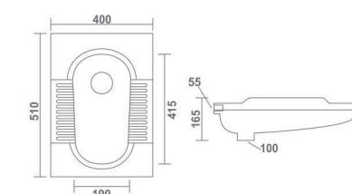
CITY PAN-20" L 510 W 400 H 165 mm
