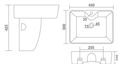
FLY L 450 W 300 H 425 mm 18" x 12"
