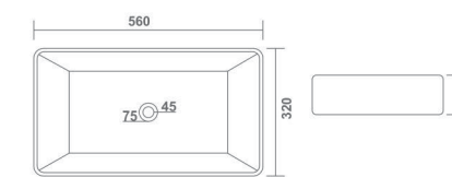
ZORO L 560 W 320 H 140 mm 22" x 13"
