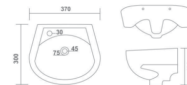
SMART L 370 W 300 H 190 mm 15" x 12"
