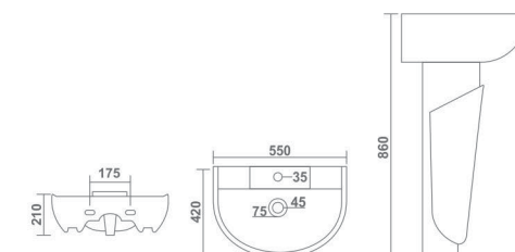
SONY L 550 W 420 H 860 mm 22" x 17"
