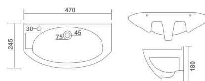
SIMON L 470 W 245 H 180 mm 19" x 10"
