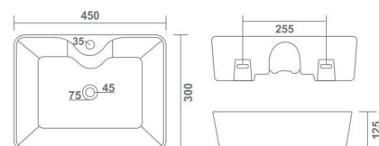
FLY L 450 W 300 H 125 mm 18" x 12"
