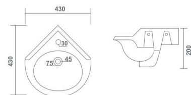
SUPER L 430 W 430 H 200 mm 17" x 17"
