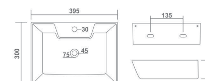
ROB L 395 W 300 H 120 mm 16" x 12"
