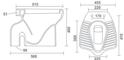
ANGLO INDIAN L 515 W 455 H 400 mm 'S' Trap
