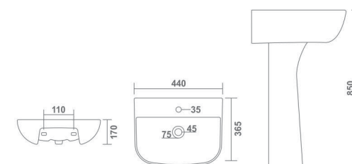
REAL L 440 W 365 H 850 mm 18" x 15"
