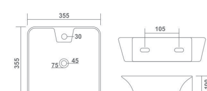
KOLAR L 355 W 355 H 100 mm 14" x 14"
